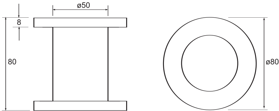
Unwound bobbin
